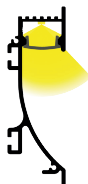
75° Negro Black -70% lumens
